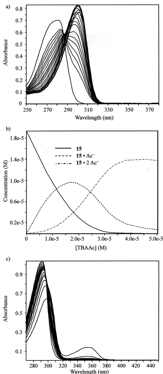
Figure 5. a) UV/Vis spectra for the titration of a solution of 15 [ 1.9 \times 10^{-5} M] with a solution of TBAAc [ 2.0 \times 10^{-4} M] in \text{CHCl}_3 ; b) distribution diagram for the chromophoric species present in solution during the titration of 15 with TBAAc; c) UV/Vis spectra for the titration of 15 ( 1.9 \times 10^{-5} M) with TBAF ( 2.0 \times 10^{-4} M) in DMSO.
